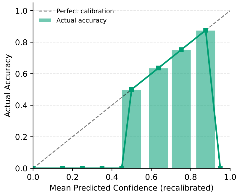
After Isotonic Recalibration (ECE = 0.000)
