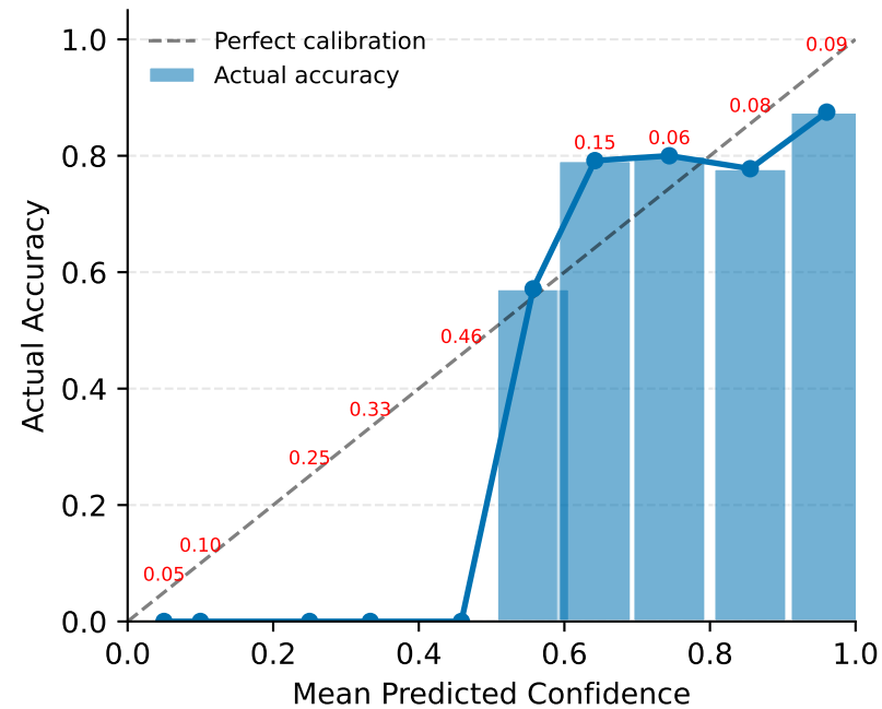
Reliability Diagram (ECE = 0.150)
